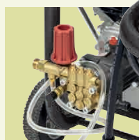
SIP AXIAL BRASS-HEADED VARIABLE PRESSURE PUMP
