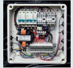
SAFETY FEATURE; 24V CONTROL CIRCUIT
