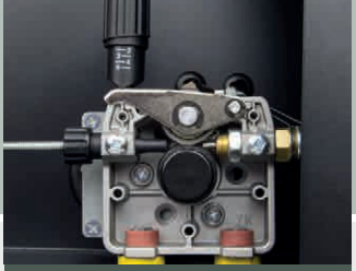
ALL-METAL 2-ROLL WIRE FEED
